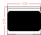
Side panels non tiltable (2pc) Padding dimension: 595 x 350 x 100 mm
